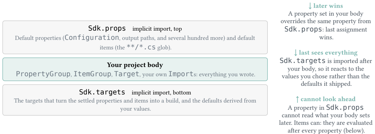
Figure 2: The import sandwich. Properties are evaluated top to bottom, so each layer can override what the layer above it set, and only the bottom layer sees every final value.
