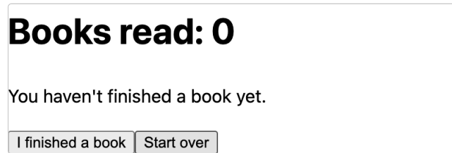
Figure 4: The React counter after the same three clicks: everything agrees
