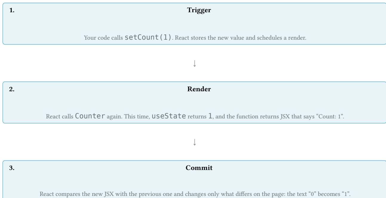
Figure 21: What React does after a setter is called. The same steps run for the first render, when the app starts.
