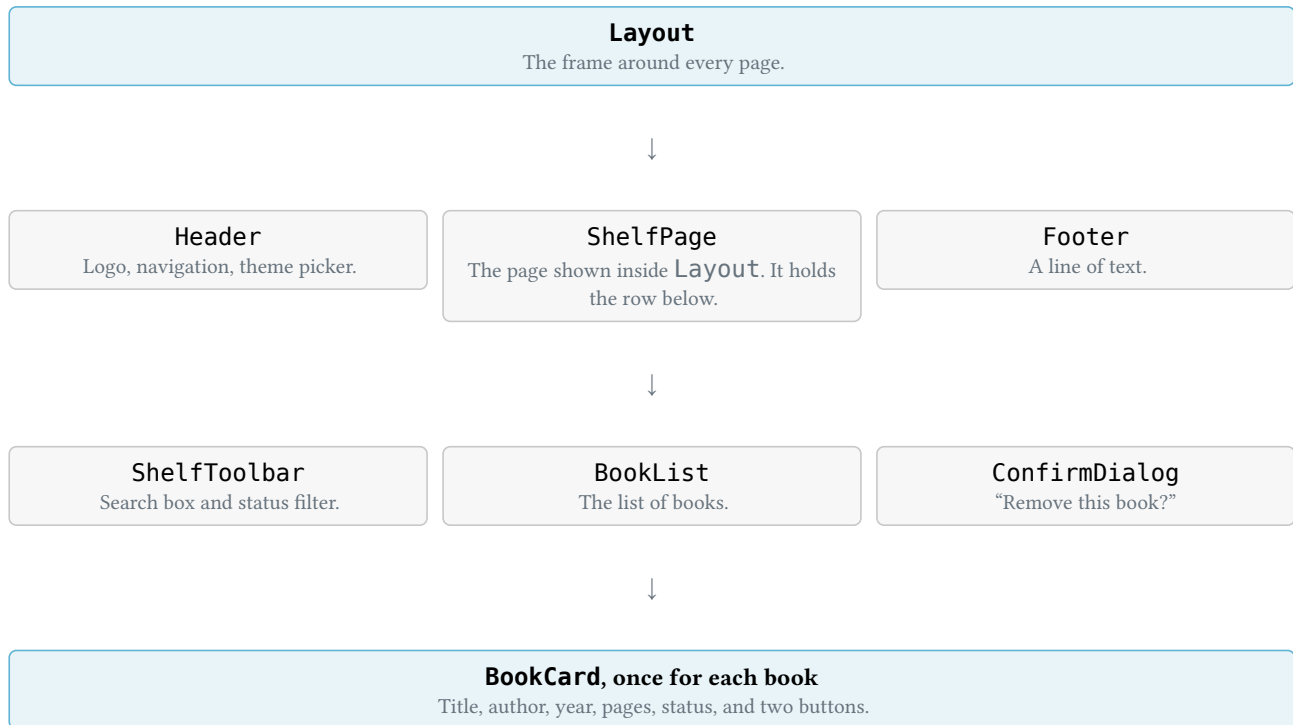
Figure 6: Shelfie’s shelf page as a tree of components
