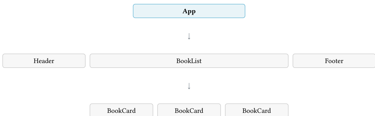
Figure 15: Shelfie's component tree. App is the parent of Header , BookList , and Footer , and BookList is the parent of the three BookCards .
