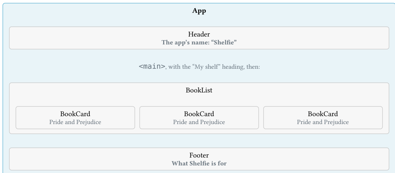
Figure 14: The Shelfie page with a box around each component. The main element and its heading belong to App itself.
