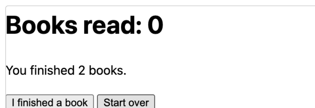
Figure 3: After “Start over”, the heading says 0 and the message still says 2
