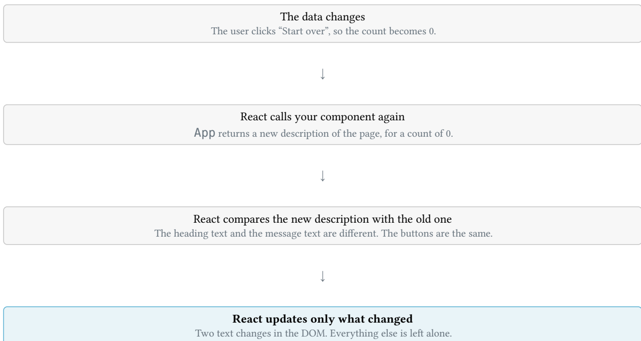
Figure 5: What happens when data changes in a React app
