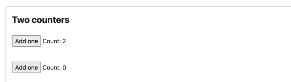
Figure 22: The first counter says 2, the second still says 0
