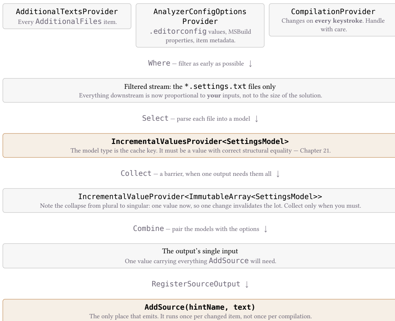
Figure 1: An incremental pipeline. Each box caches its own output; a box re-runs only when something it depends on produces a value that is not equal to last time's. The equality in that sentence is Chapter 21, and it is the part that goes wrong.
